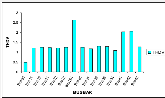
Fig. 7 The effects of harmonic source at bus 201 to THDV at various busbar
