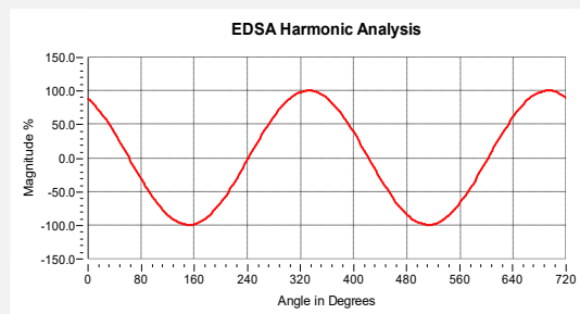
Fig 4 Distorted Current Waveform at Bus 50
